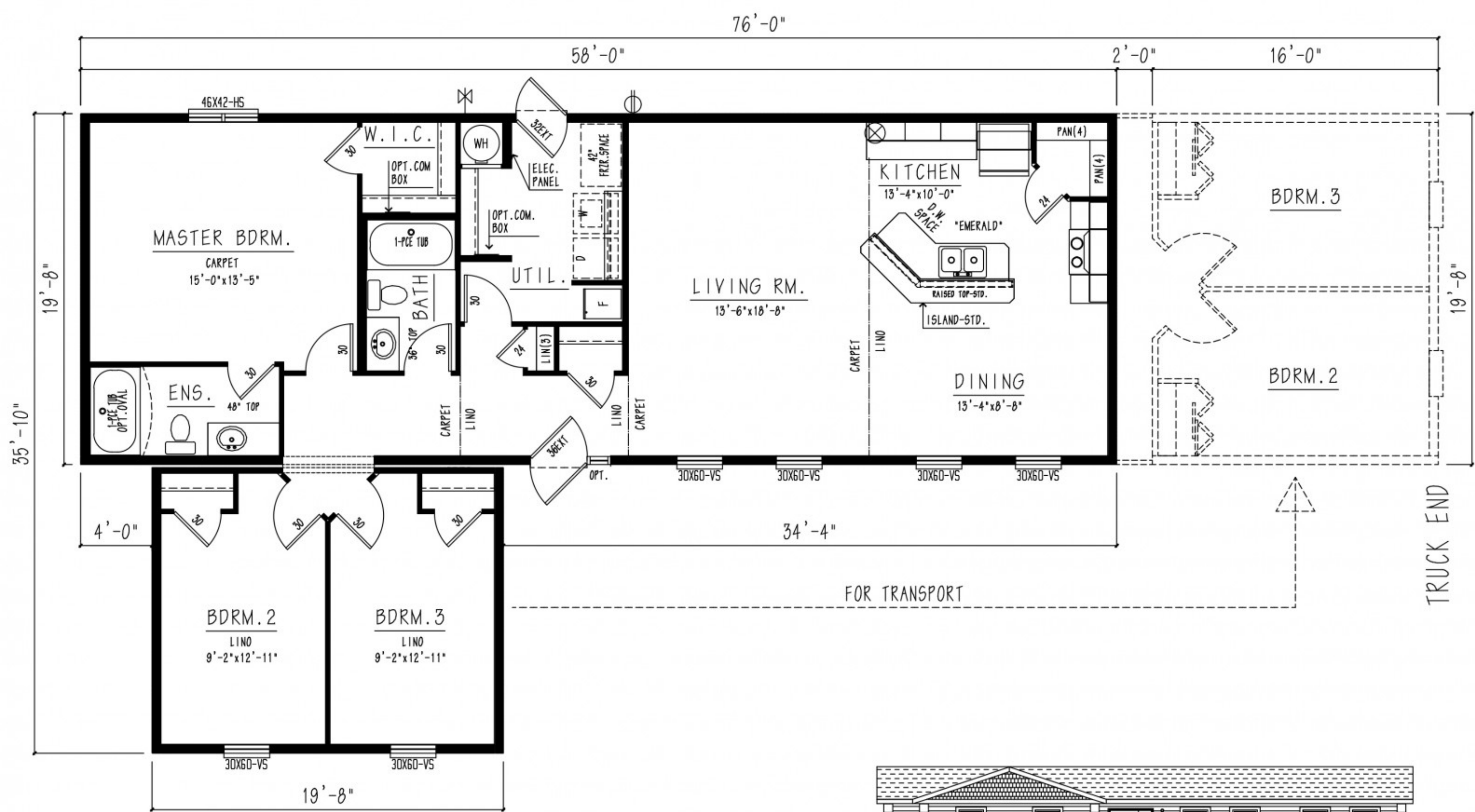
FLOOR PLAN SELF-CONTAINED [1455 SQ.FT.]
