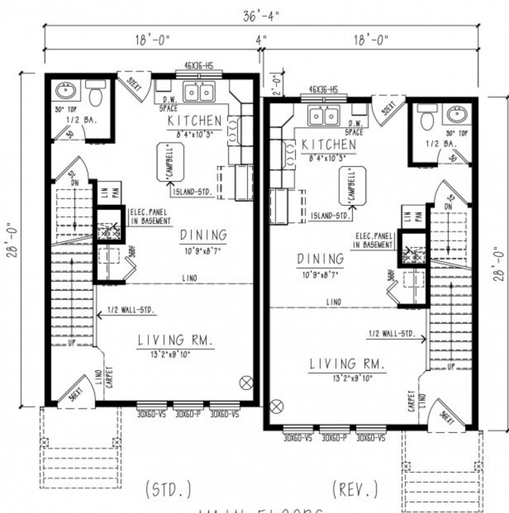
MAIN FLOORS [APPROX. 504 SQ. FT. PER SIDE]
