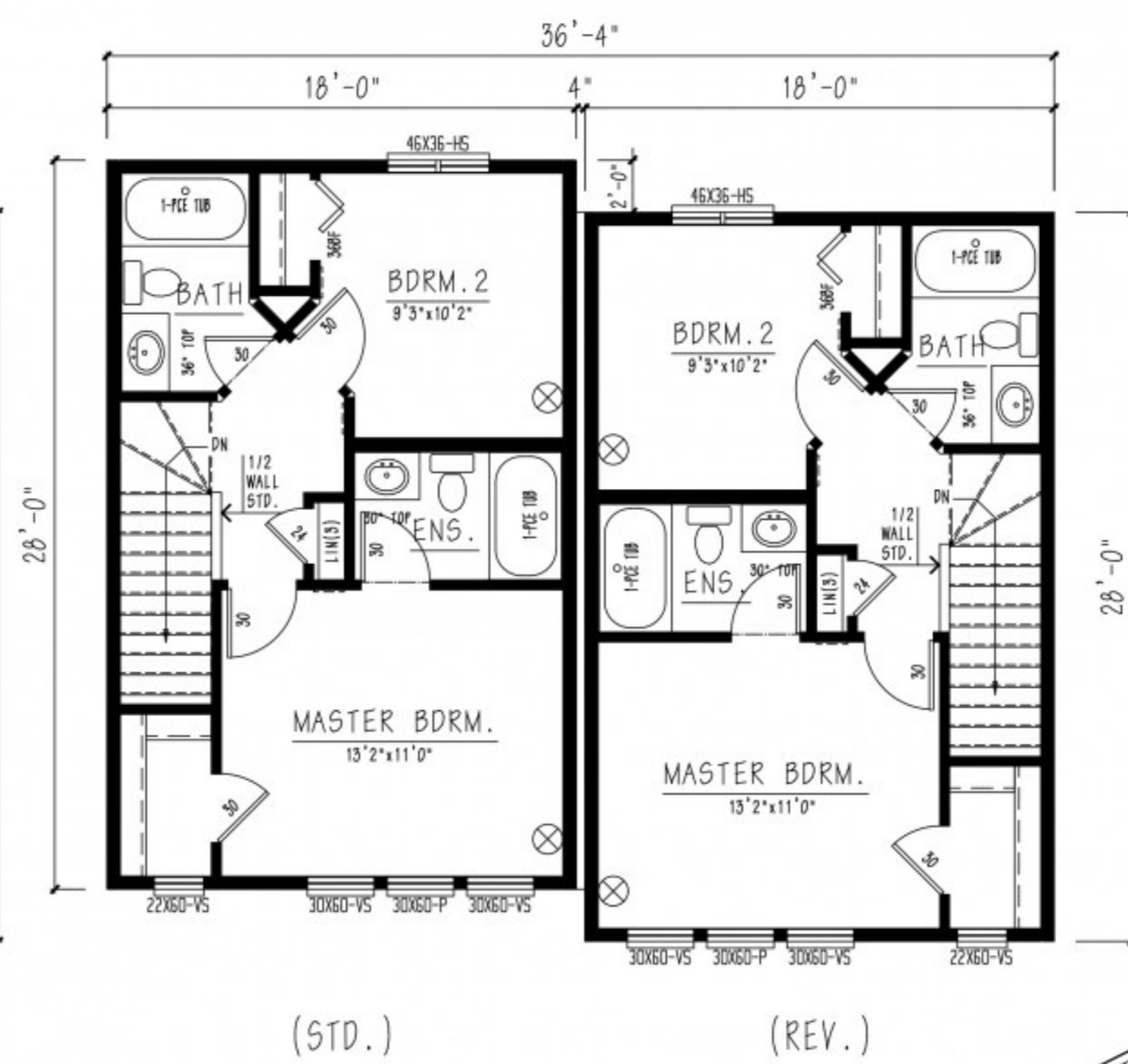
UPPER FLOORS [APPROX. 504 SQ. FT. PER SIDE]
