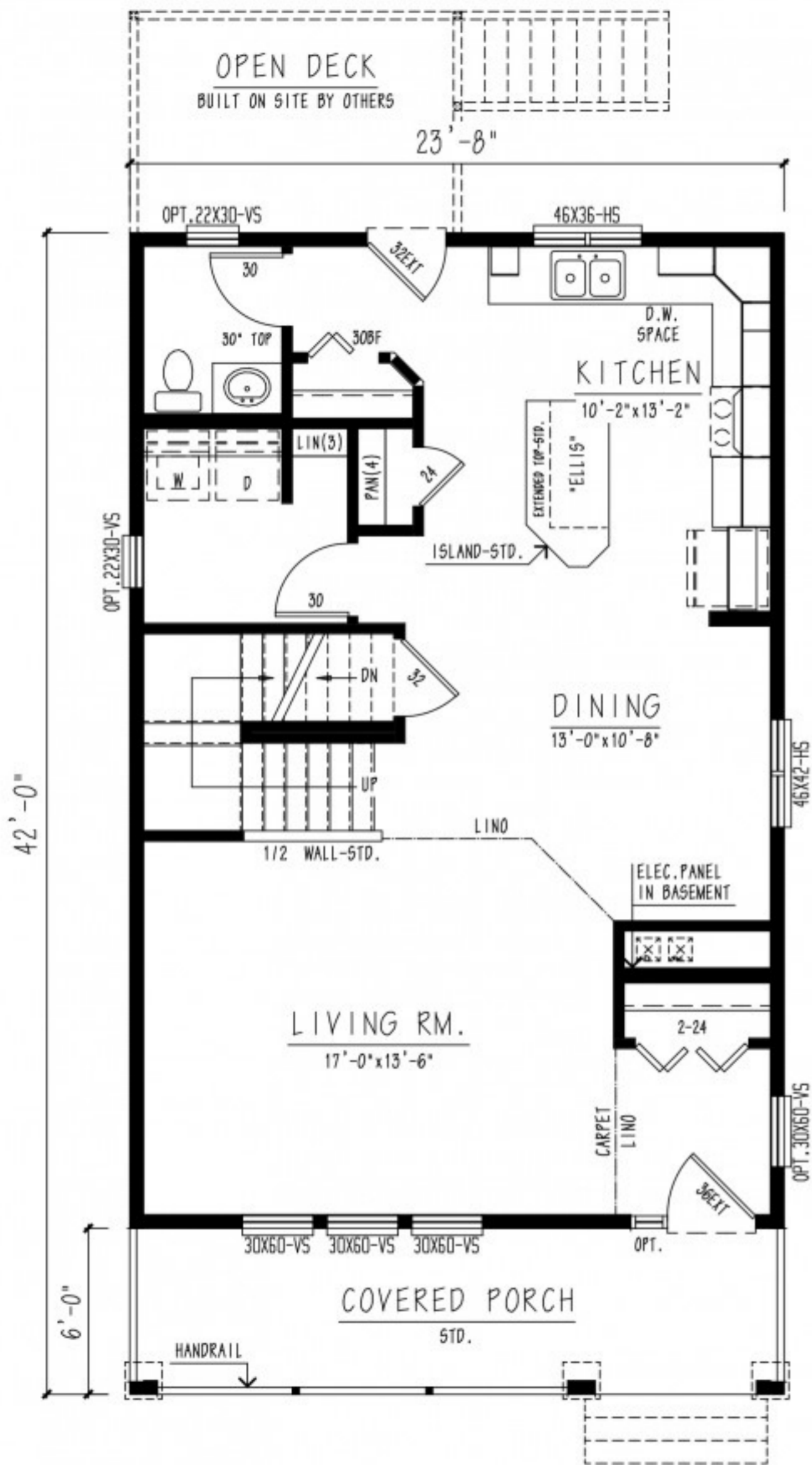
MAIN FLOOR [APPROX. 852 SQ. FT.]
