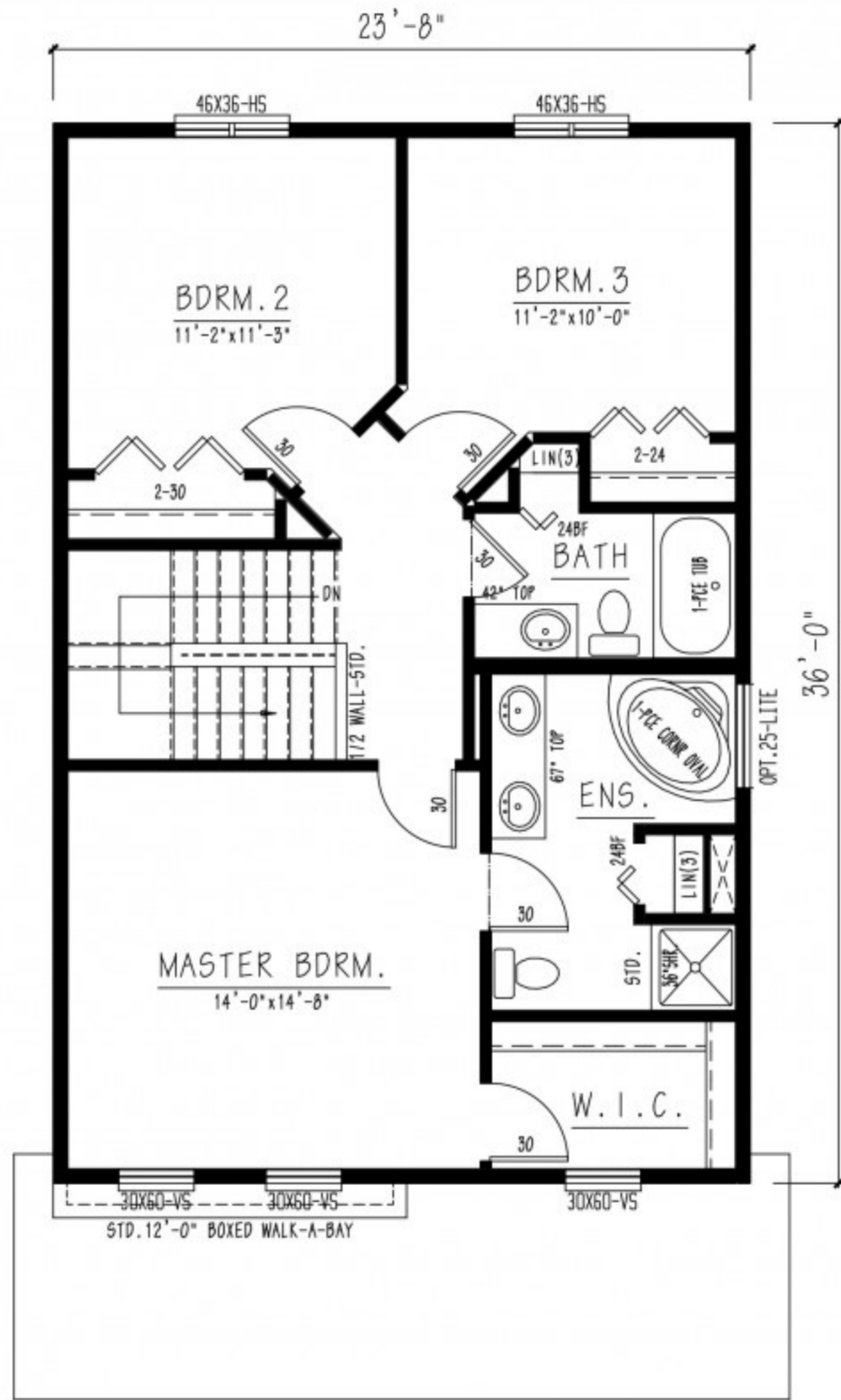
UPPER FLOOR [APPROX. 866 SQ. FT.]
