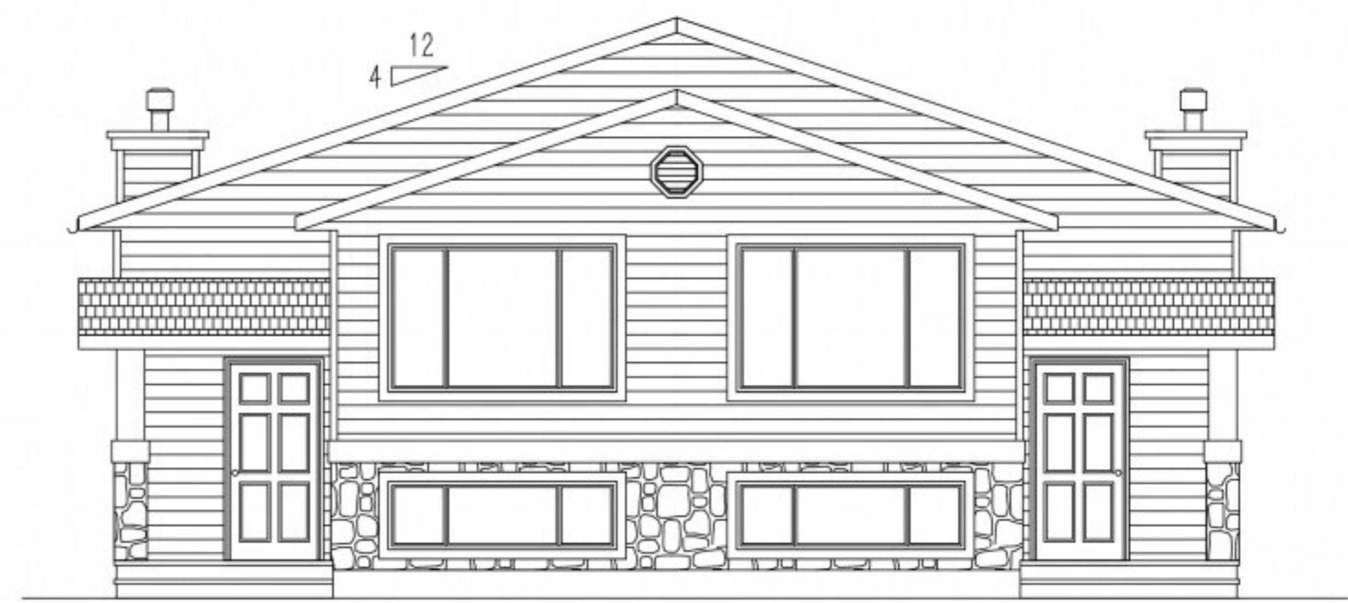
the "BRADFORD-DUPLEX" [APPROX. 968 SQ. FT. PER SIDE]
