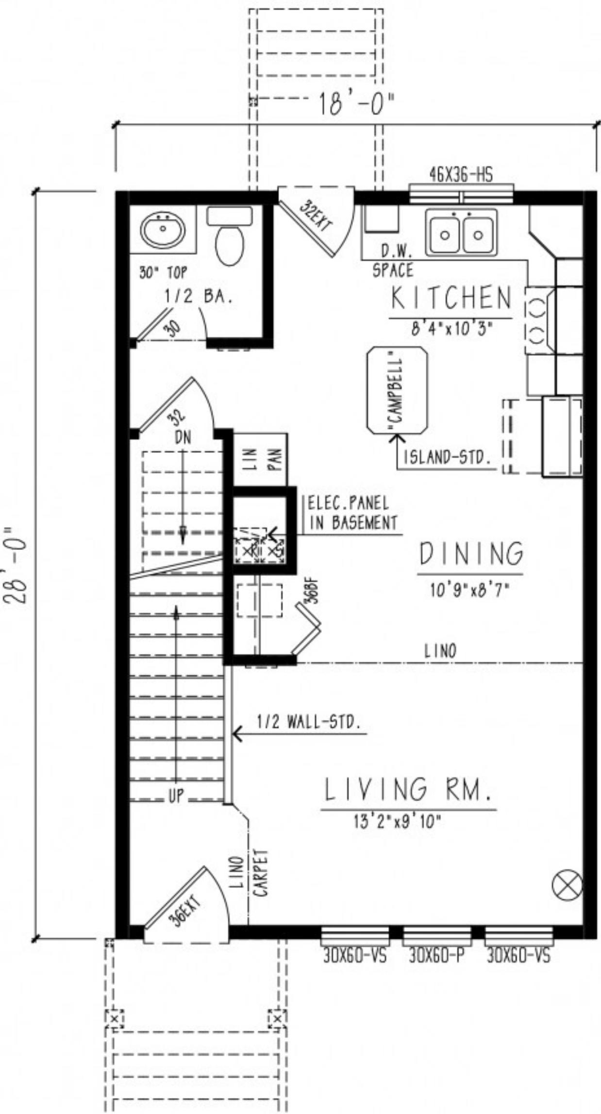
MAIN FLOOR [APPROX. 504 SQ. FT.]
