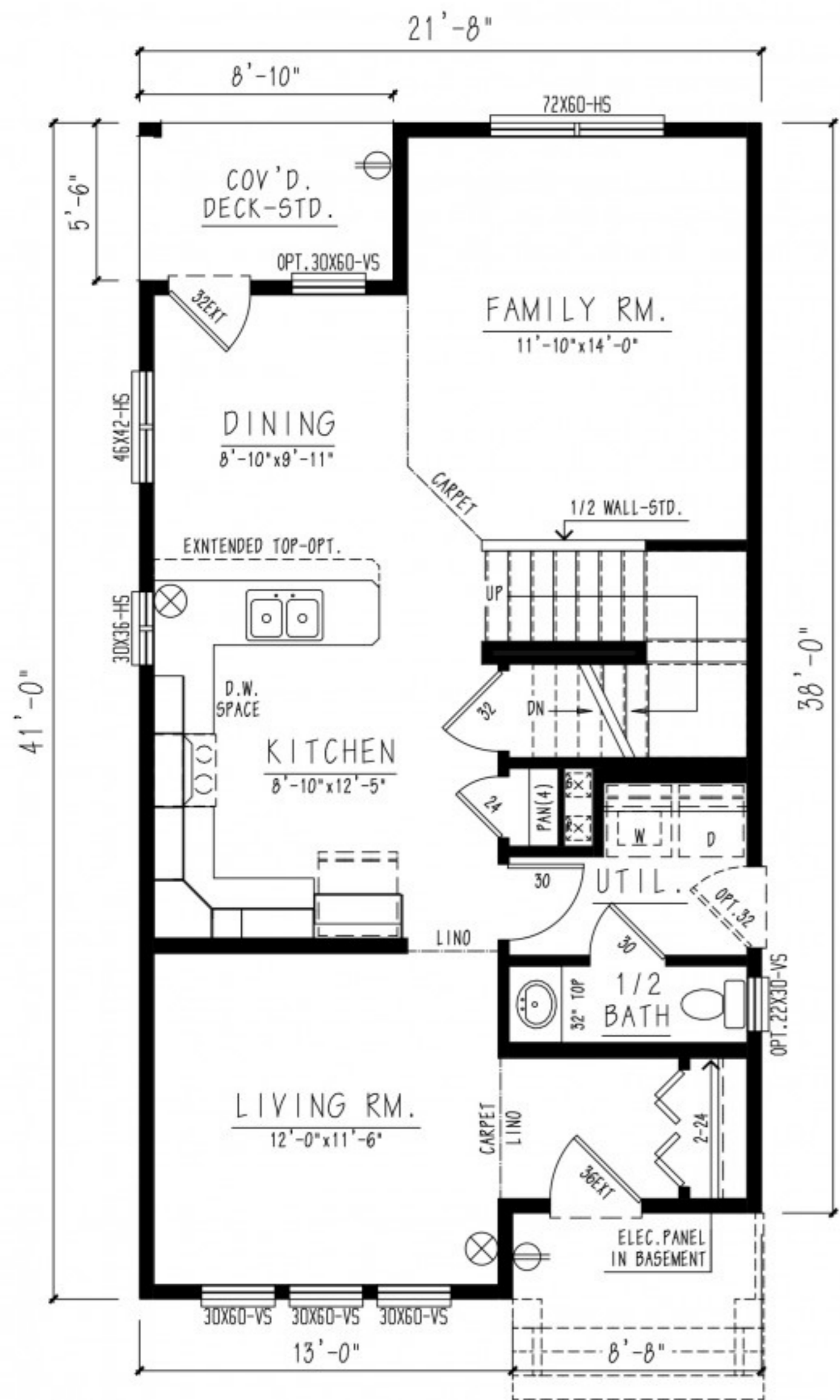
MAIN FLOOR [APPROX. 814 SQ. FT.]
