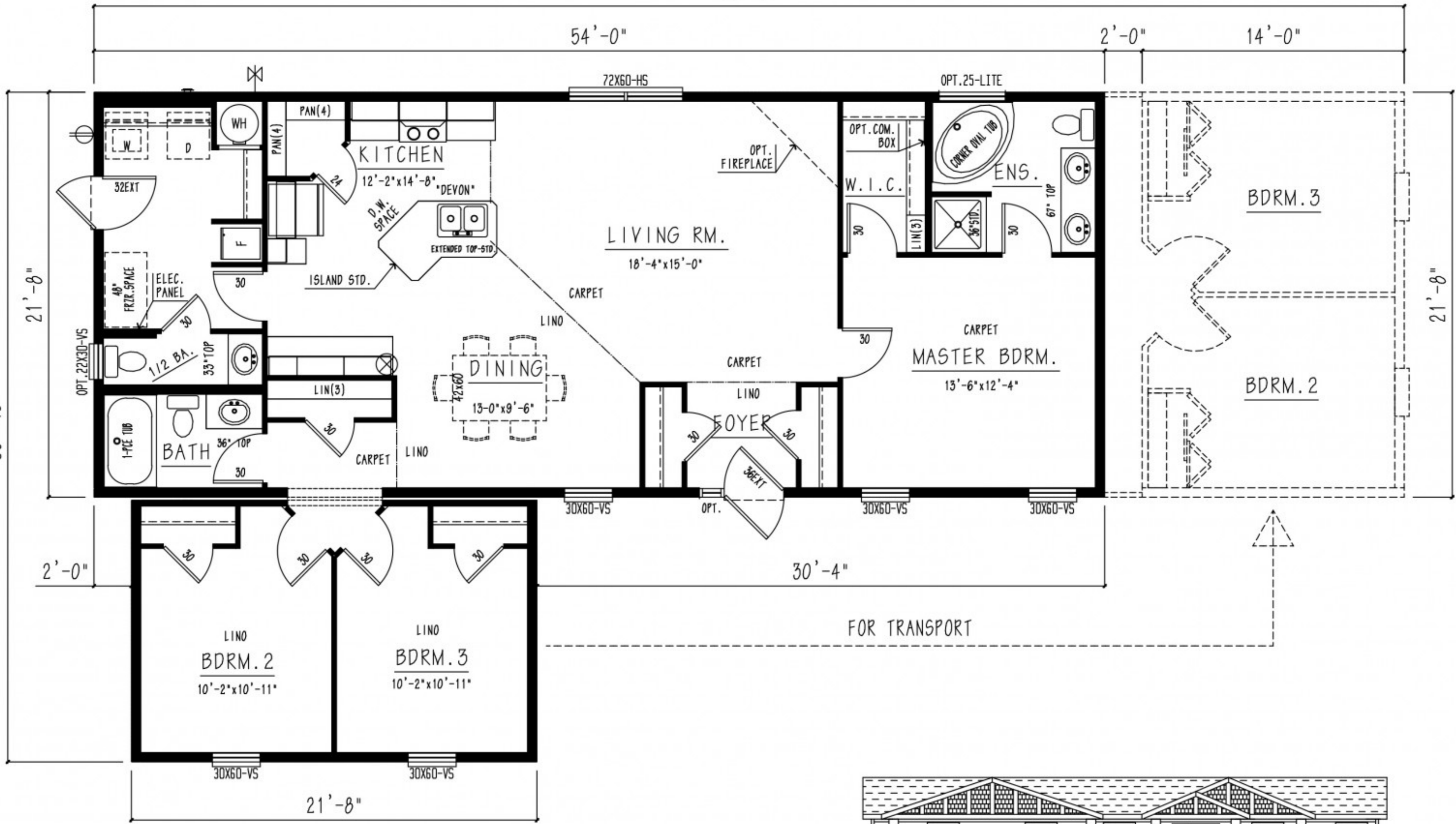
FLOOR PLAN SELF-CONTAINED [1473 SQ.FT.]
