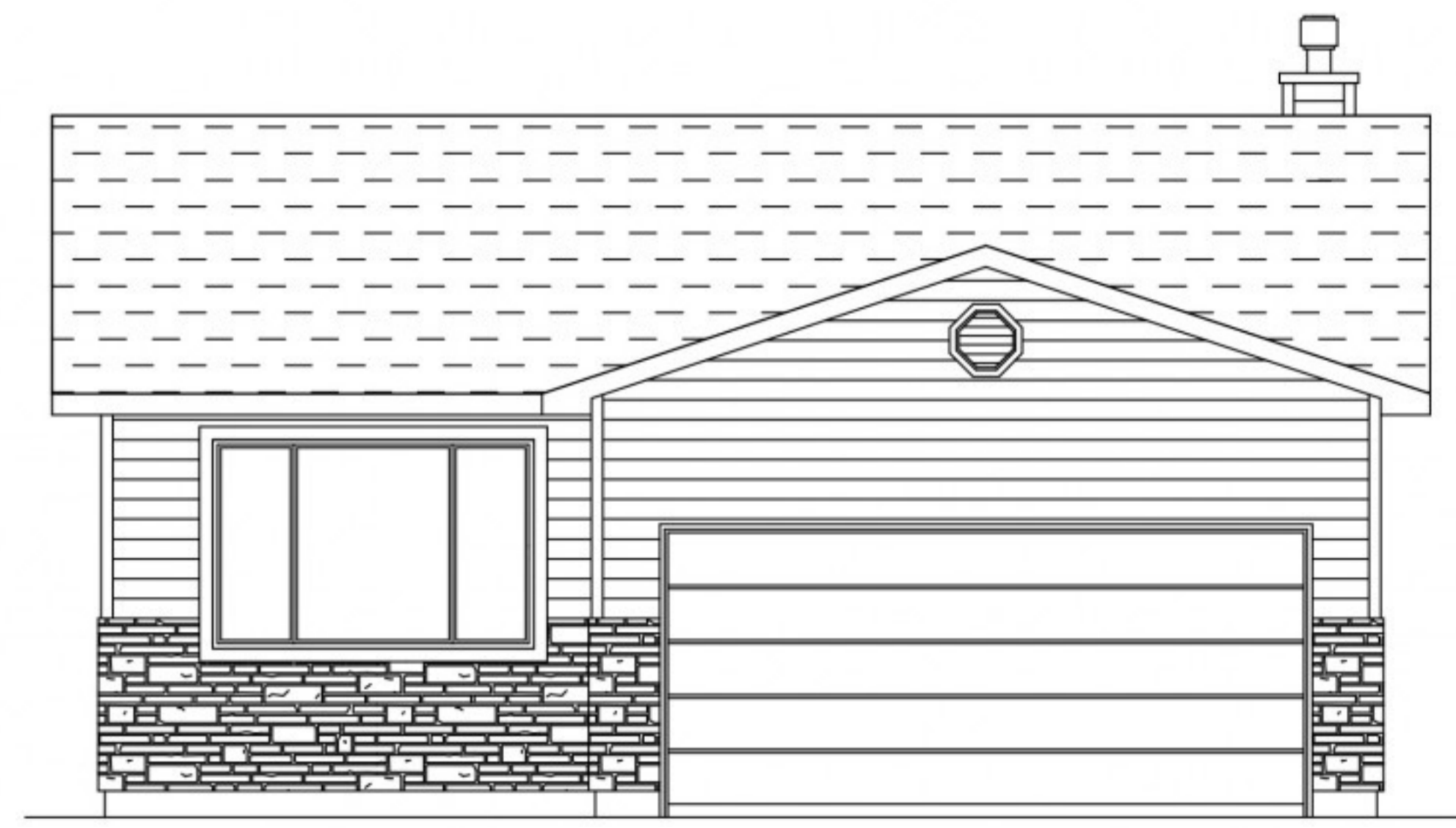
the "KODIAK" [APPROX. 1258 SQ. FT.]
